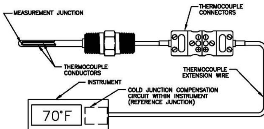
FIGURE 3: THERMOCOUPLE SENSOR CONSTRUCTIONS
