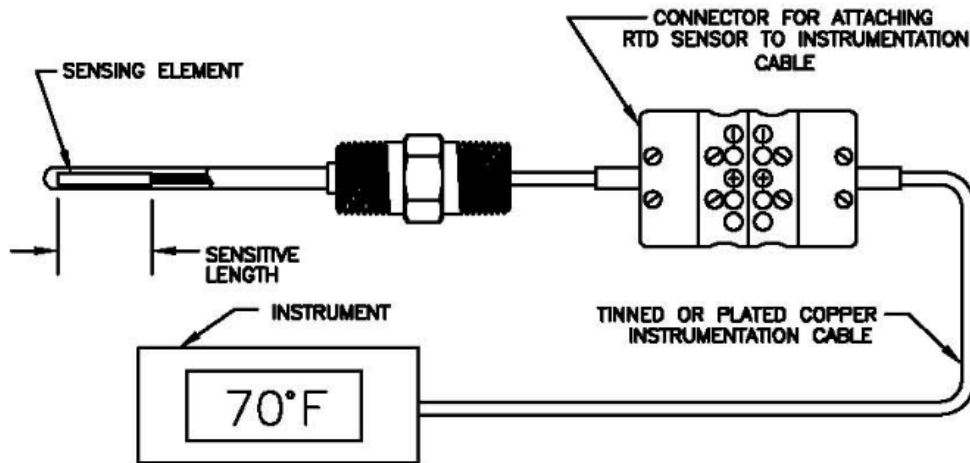
FIGURE 2: RTD SENSOR CONSTRUCTIONS
