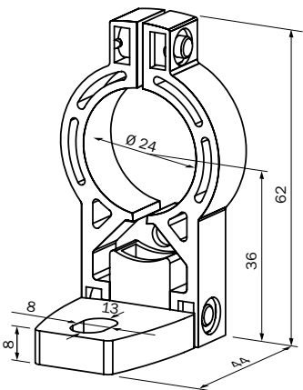
Dimensional drawing
