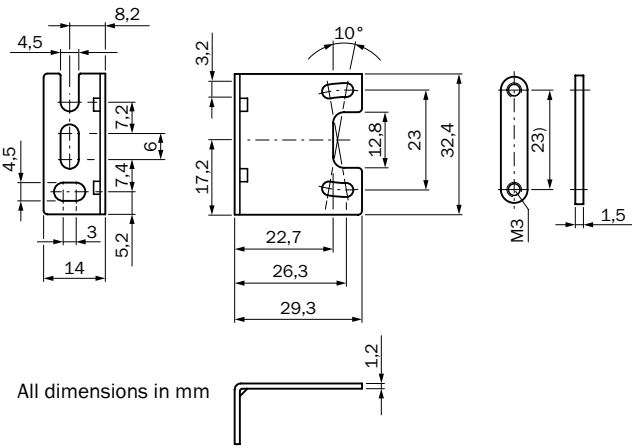
Dimensional drawing
