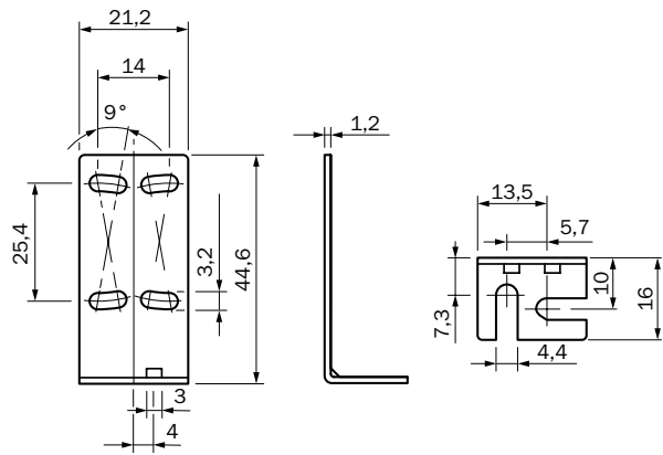
Dimensional drawing
