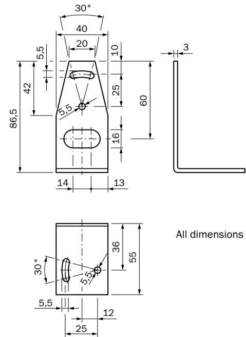
Dimensional drawing
