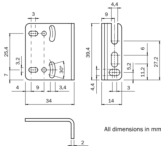
Dimensional drawing
