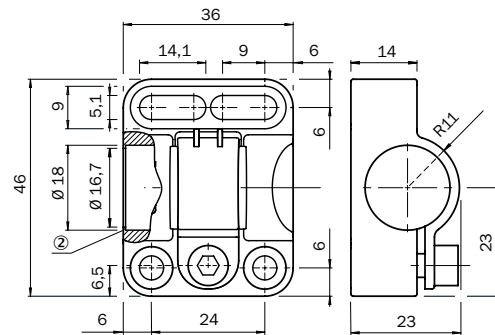
Dimensional drawing
