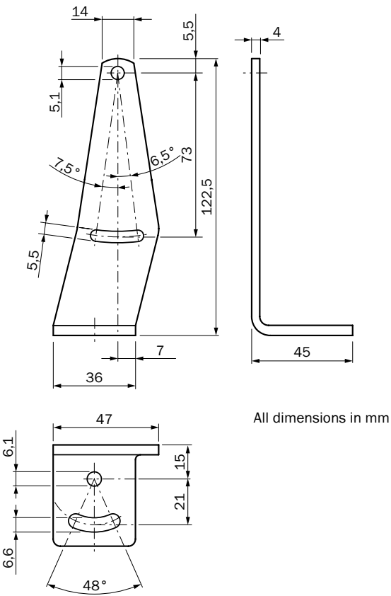
Dimensional drawing
