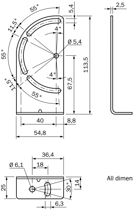
Dimensional drawing
